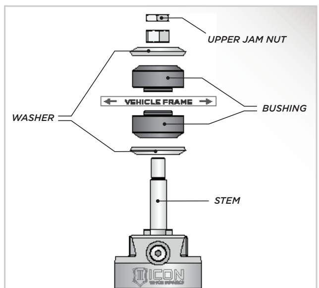
HD STEM BUSHING DIAGRAM
